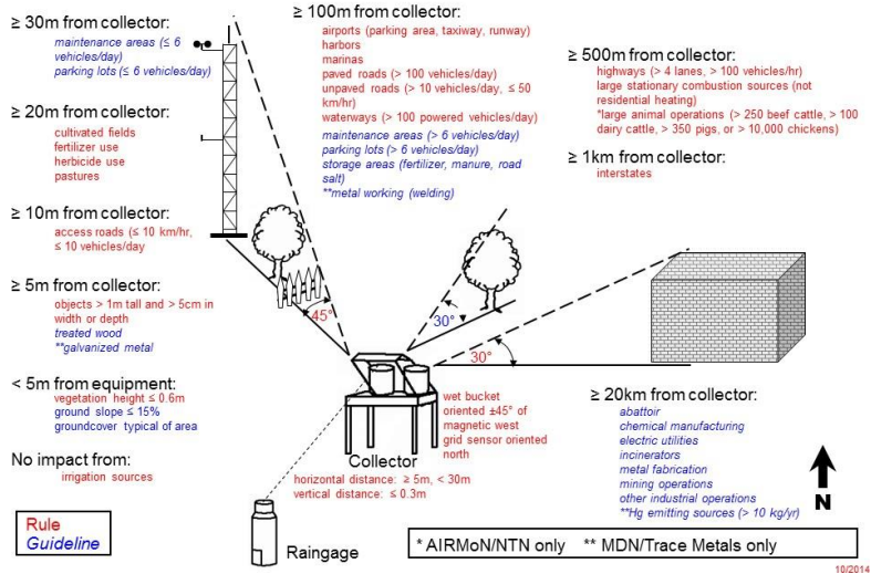
Figure 6. NADP general siting criteria for wet deposition sampling site. Note in this design, influence from local sources is intended to be eliminated—providing only the measurement of regional rain events.
